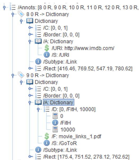
Internal view of the PDF
